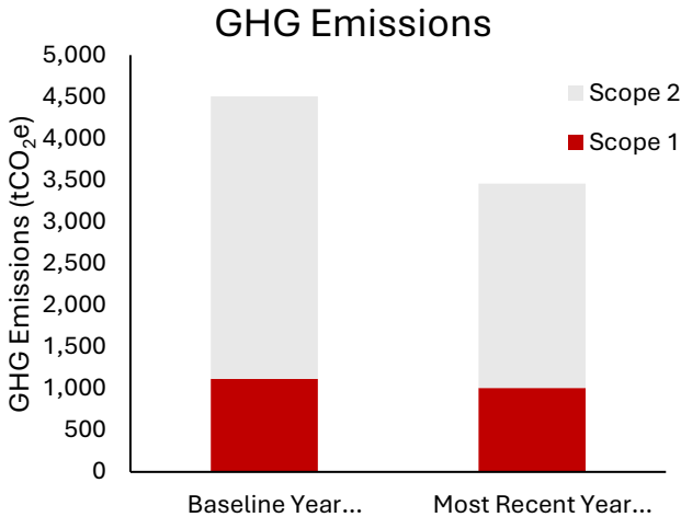
Figure 1: A summary of the GHG emissions as per the GHG Protocol.
